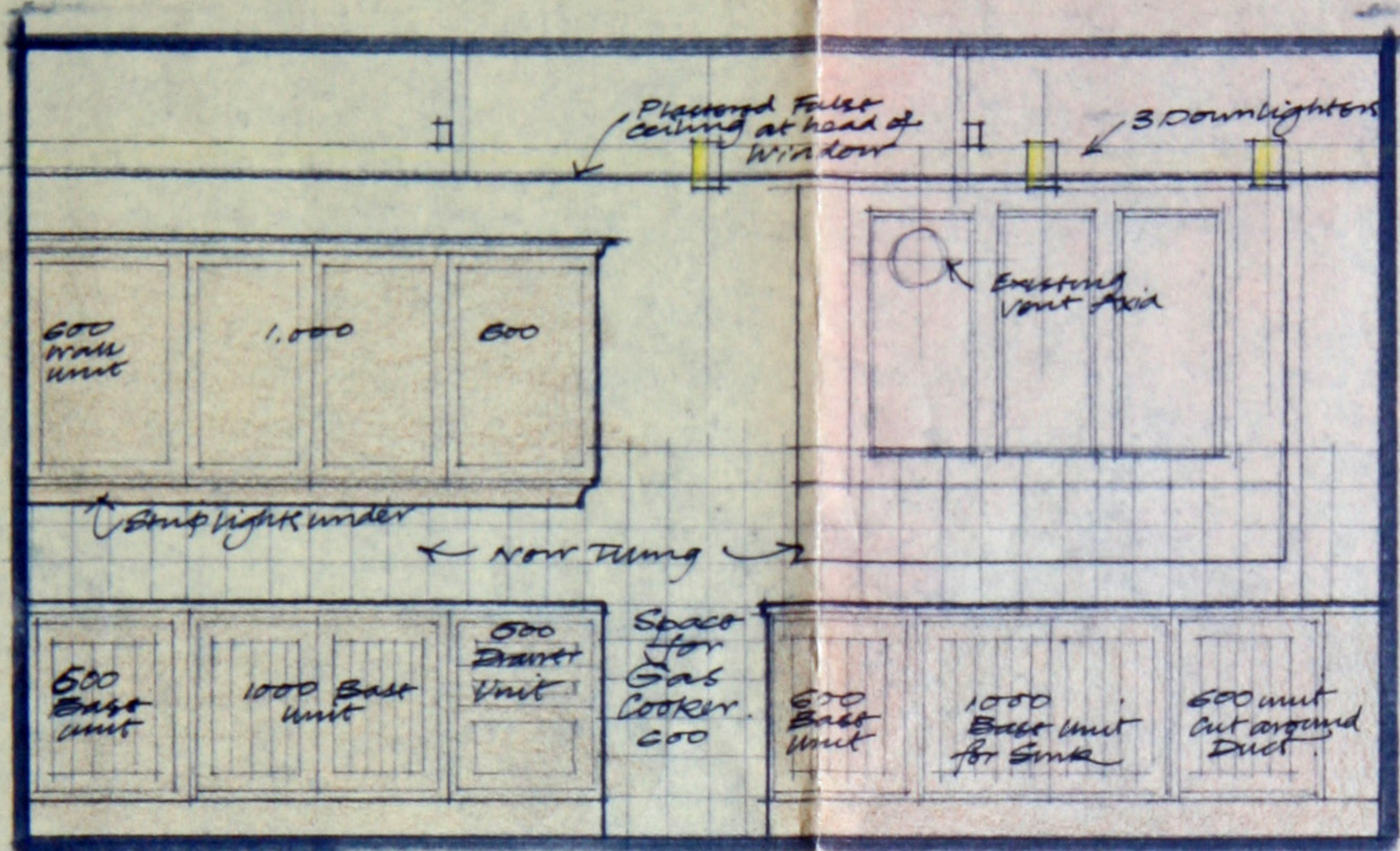
Elevation 1/2 to 1'-0"
